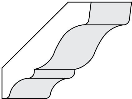
#49G0 [11/16" x 3-1/4"] Poplar • Oak
